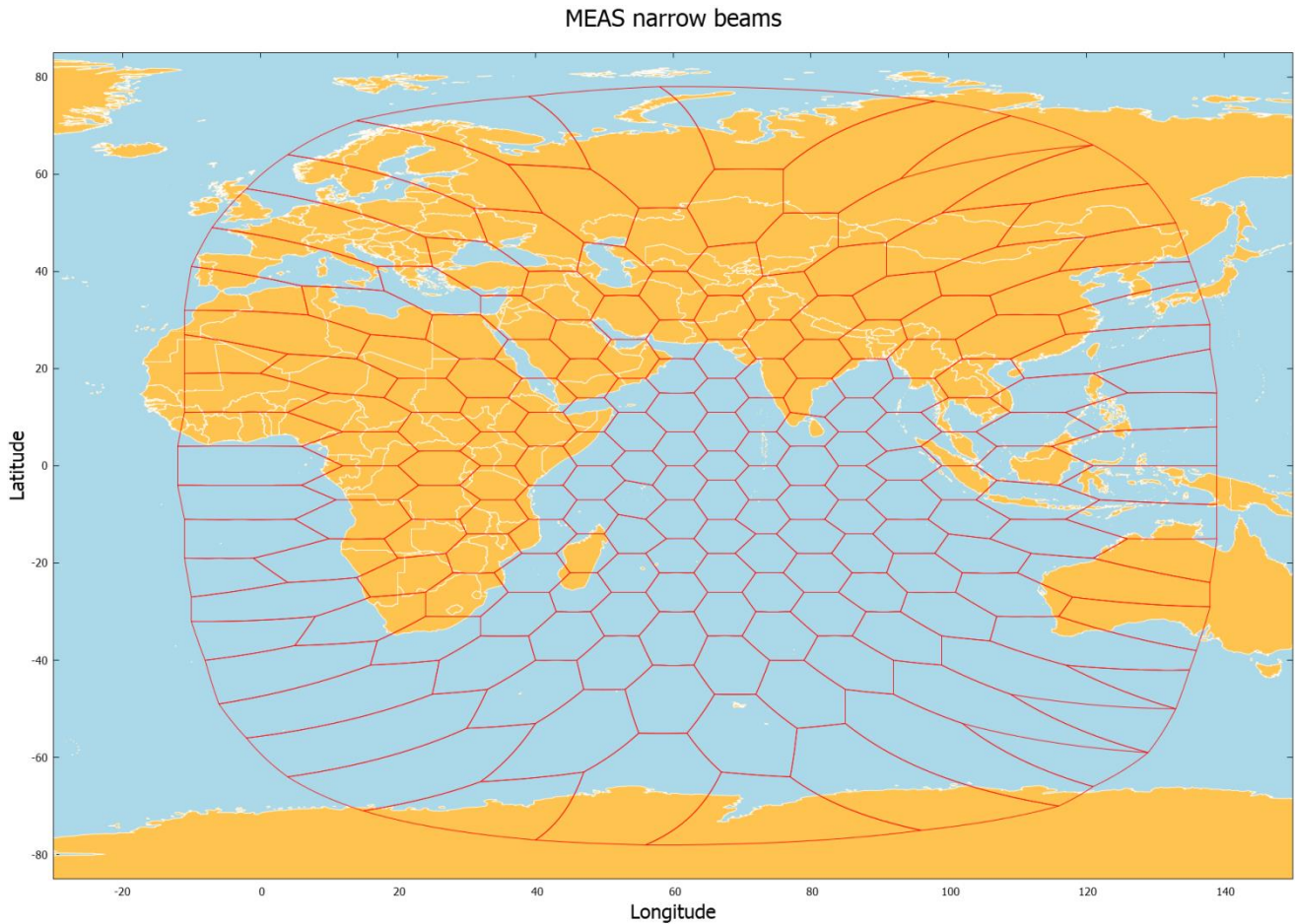
Figure 4-6: MEAS narrow spot beams 12
